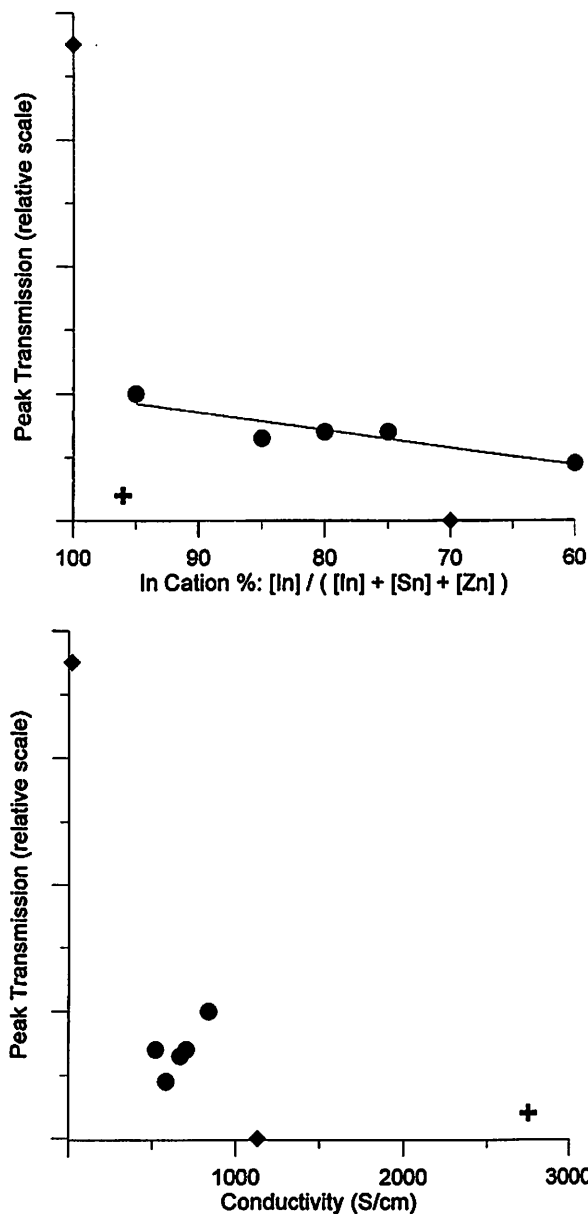
Figure 5. Plot of peak (500 nm) transmittance versus cation % In (a, top) and versus conductivity (b, bottom). Samples shown are (◆) cosubstituted copper-quenched including pure In 2 O 3 , (●) air-quenched cosubstituted, (+) 4 cation % Sn ITO.
