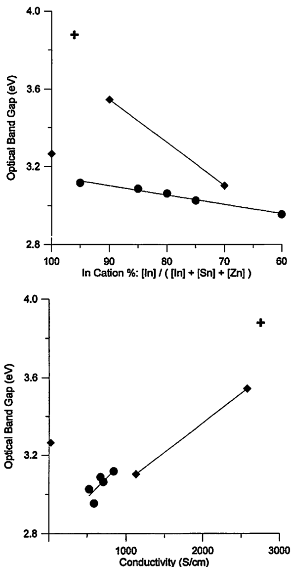
Figure 4. Optical bandgap versus cation % In (a, top) and versus conductivity (b, bottom). Samples shown are (◆) cosubstituted copper-quenched including pure In 2 O 3 , (●) air-quenched cosubstituted, (+) 4 cation % Sn ITO.
