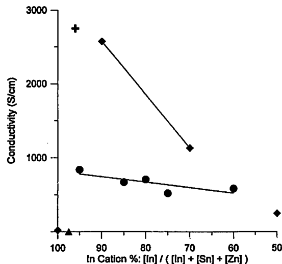
Figure 2. Conductivity versus cation % In. Samples shown are (♦) cosubstituted copper-quenched including In 2 O 3 , (●) air-quenched cosubstituted, (+) 4 cation % Sn ITO, (▲) 97.8 cation % In/2.2 cation % Zn oxide.
