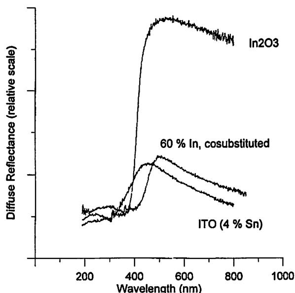
Figure 3. Diffuse reflectance spectra of \text{In}_2\text{O}_3 , ITO, and cosubstituted \text{In}_2\text{O}_3 .
