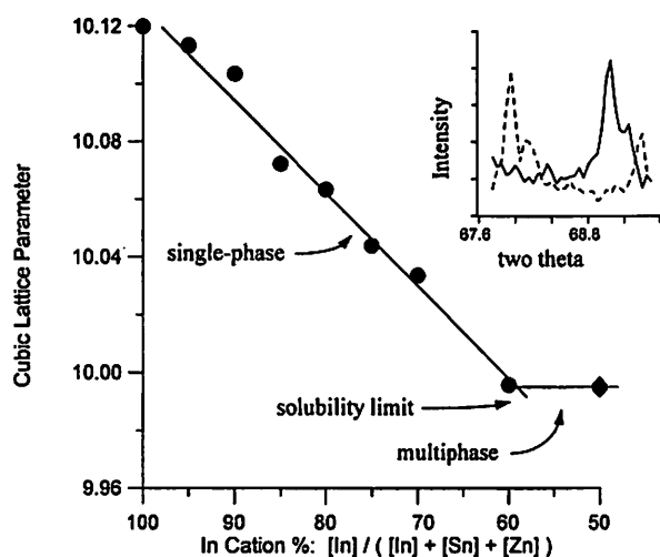
Figure 1. Lattice parameter versus cation % In. The sloping region is single phase. The horizontal line is three phase. The inset powder pattern shows the pronounced two theta shift of the 721 peak between In 2 O 3 (dashed line) and In 1.2 Sn 0.4 Zn 0.4 O 3 (solid line).
