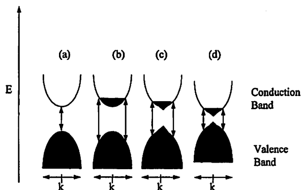
Figure 6. Schematic band structure diagram for cosubstituted \text{In}_2\text{O}_3 . (a) The direct bandgap of an undoped semiconductor, e.g., pure \text{In}_2\text{O}_3 . (b) In degenerate doped semiconductors such as ITO, the filling of states causes the direct bandgap to increase (Moss–Burstein shift). (c) Many-body effects in ITO cause a partial bandgap narrowing but the overall bandgap is still larger than in \text{In}_2\text{O}_3 . (d) Creation of acceptor–donor pairs in cosubstituted \text{In}_2\text{O}_3 causes a dramatic bandgap narrowing effect which often makes the overall bandgap smaller than in pure \text{In}_2\text{O}_3 .
